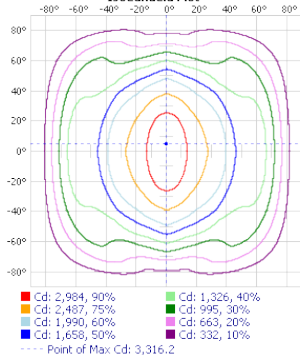
IsoCandela Plot
