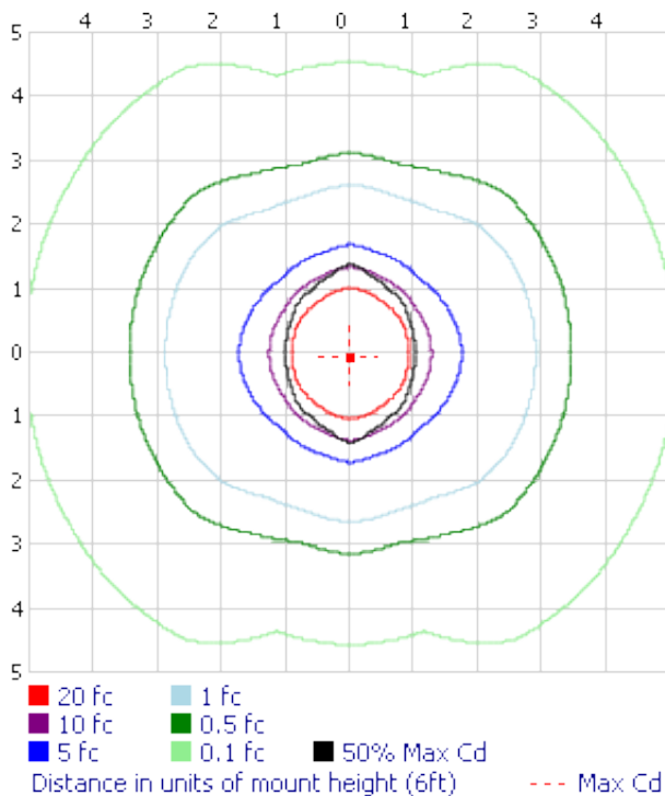
Isolux Plot
