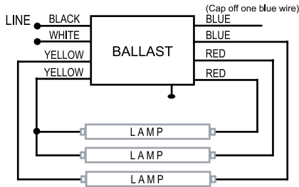
THREE LAMP
