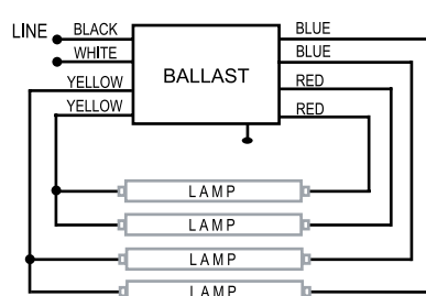
FOUR LAMP
