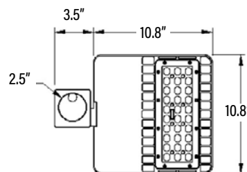
Slip Fitter with Item#: 83505, 83509
