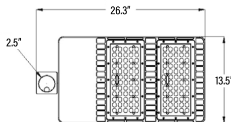
Slip Fitter with Item#: 83520, 83522, 83547, 83548
