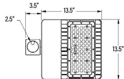
Slip Fitter with Item#: 83511, 83512, 83517, 83545, 83546
