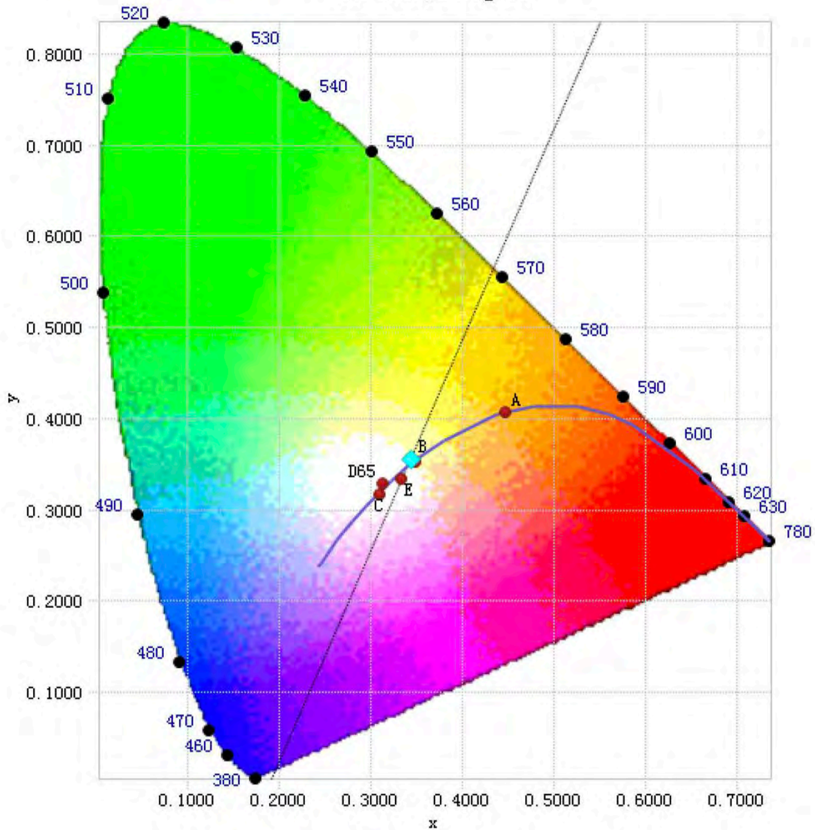
Chart 2: Chromaticity Diagram per Sphere - Spectroradiometer Method
