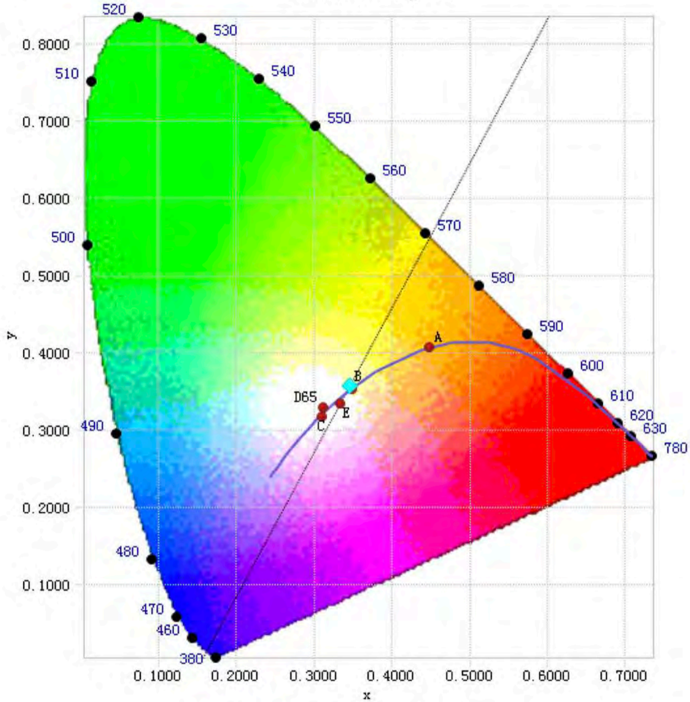
Chart 2: Chromaticity Diagram per Sphere - Spectroradiometer Method
