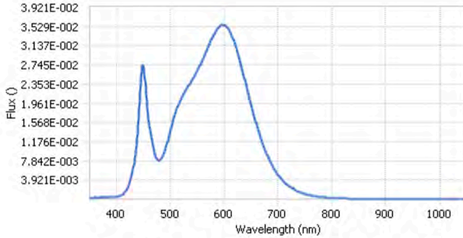
Chart 1: Spectral Power Distribution
