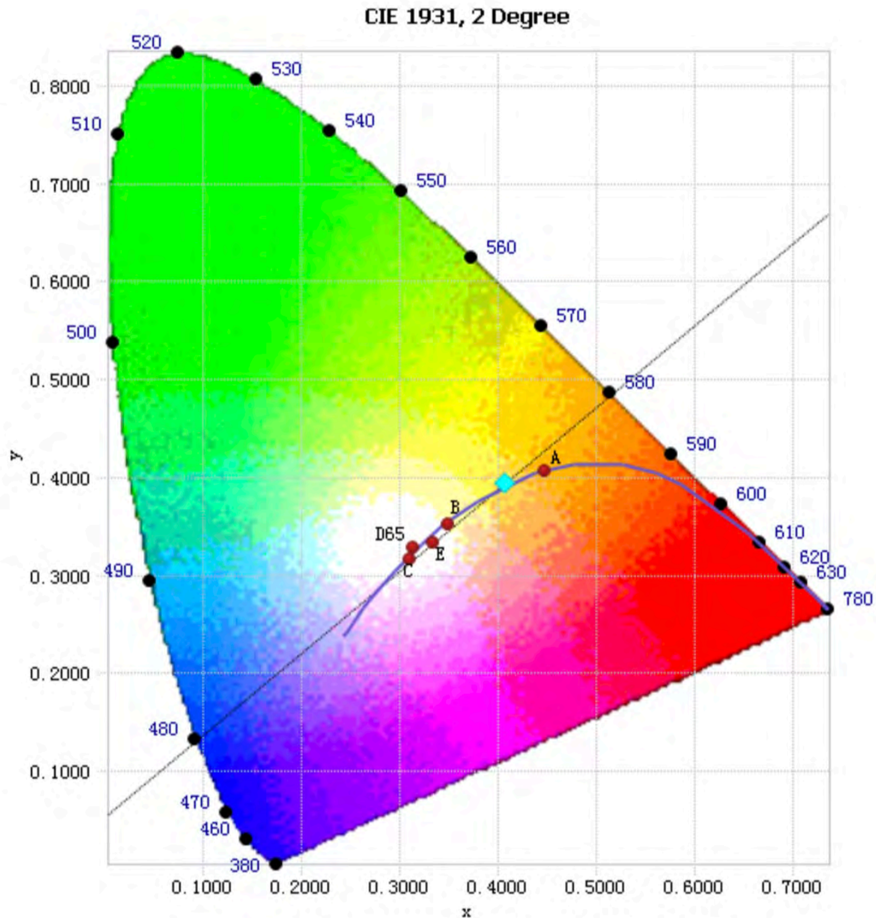
Chart 2: Chromaticity Diagram per Sphere - Spectroradiometer Method
