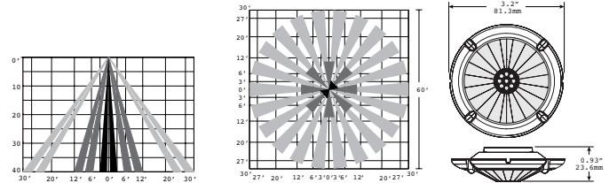
FSP-L4 360° lens, maximum coverage 60' diameter from 40' height
