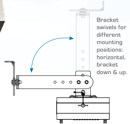
MOUNTING KIT INCLUDED
